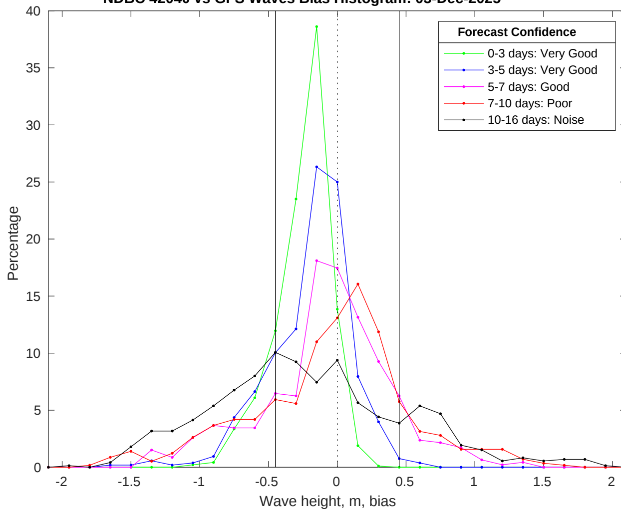
NDBC 42040 vs GFS Waves Bias Histogram: 03-Dec-2025
