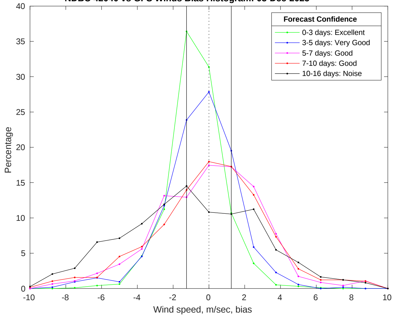
NDBC 42040 vs GFS Winds Bias Histogram: 03-Dec-2025
