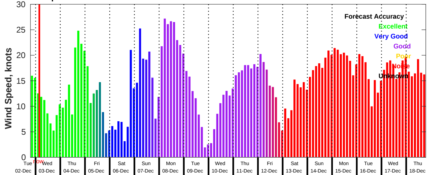
GFS Wind Speed Forecast for NDBC 42040 from 02-Dec-2025 19:00:00 to 18-Dec-2025 19:00:00
