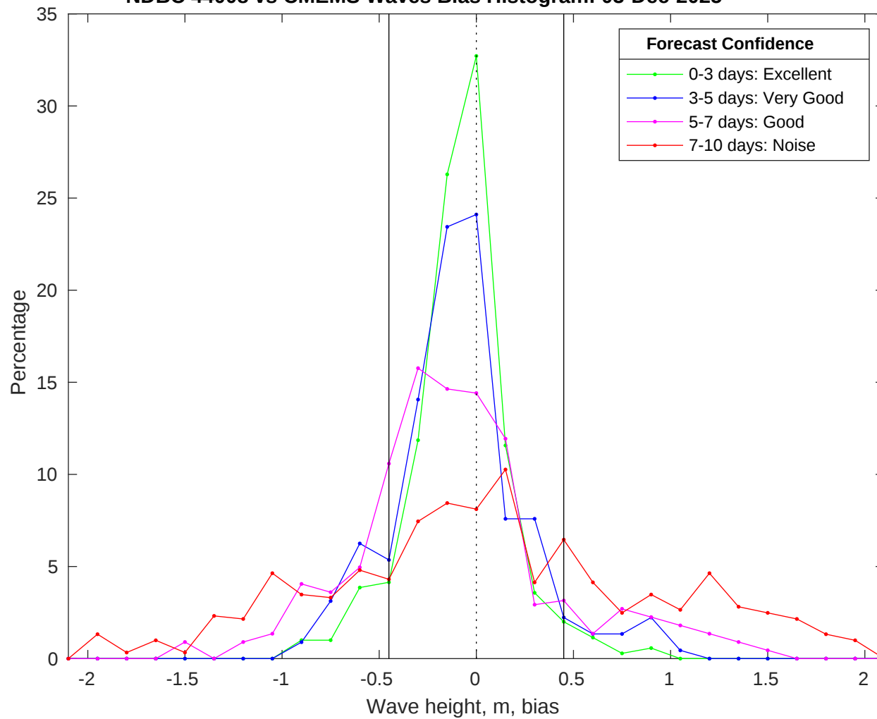
NDBC 44008 vs CMEMS Waves Bias Histogram: 03-Dec-2025
