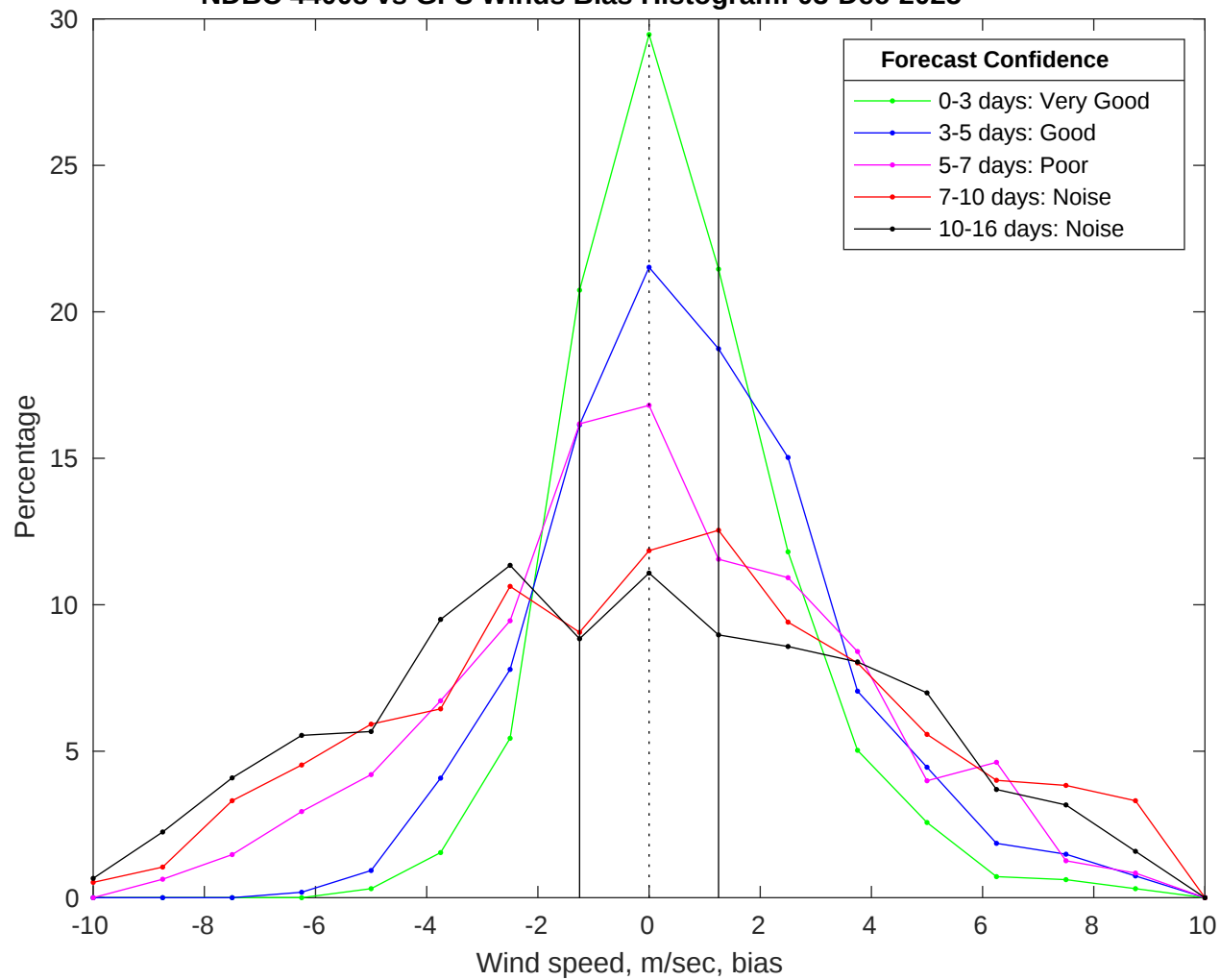
NDBC 44008 vs GFS Winds Bias Histogram: 03-Dec-2025
