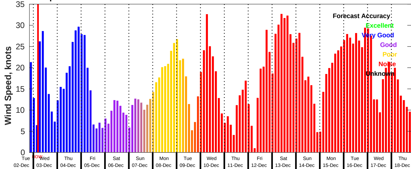
GFS Wind Speed Forecast for NDBC 44008 from 02-Dec-2025 20:00:00 to 18-Dec-2025 20:00:00
