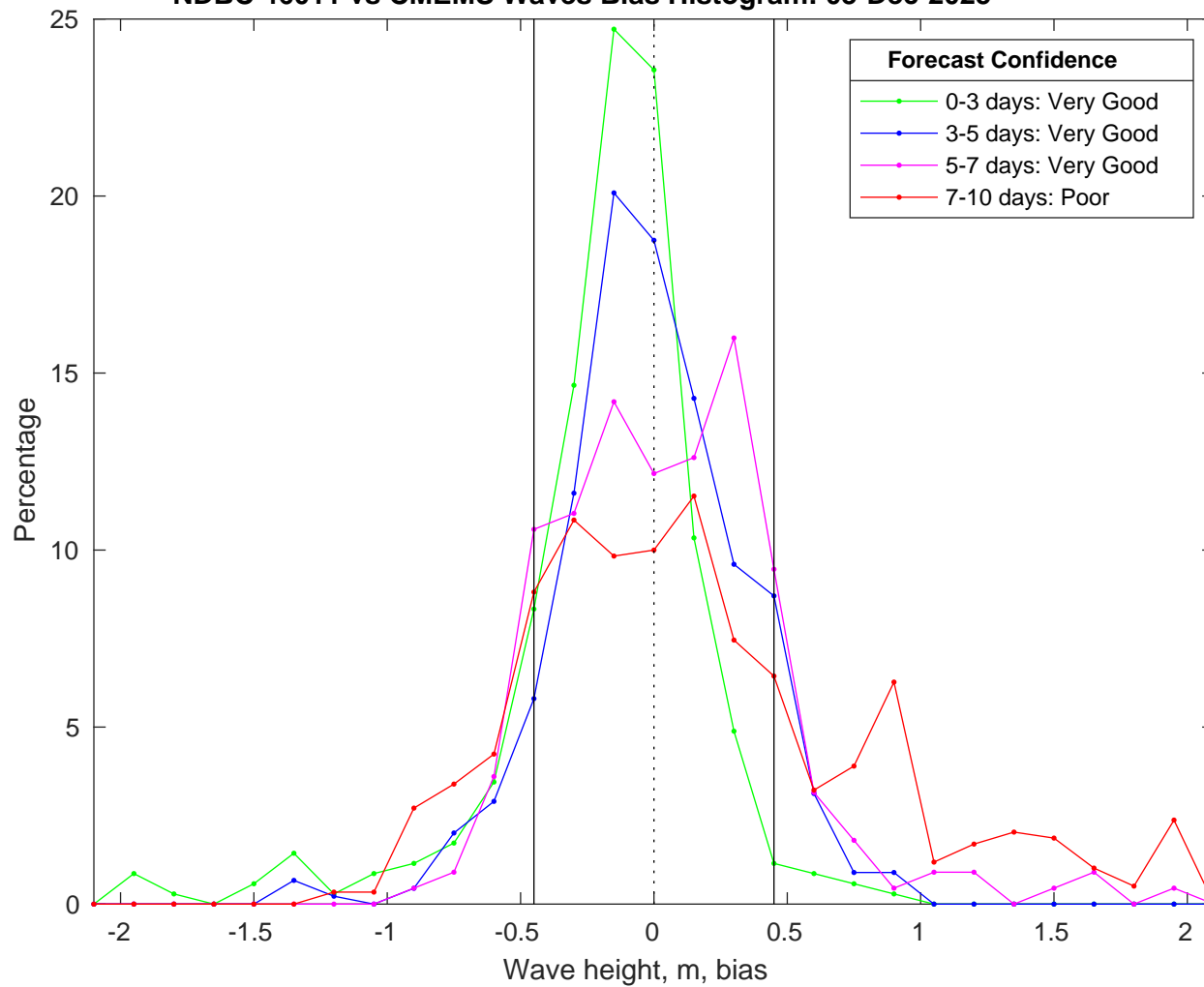
NDBC 46011 vs CMEMS Waves Bias Histogram: 03-Dec-2025
