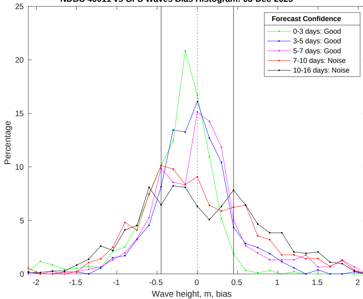
NDBC 46011 vs GFS Waves Bias Histogram: 03-Dec-2025
