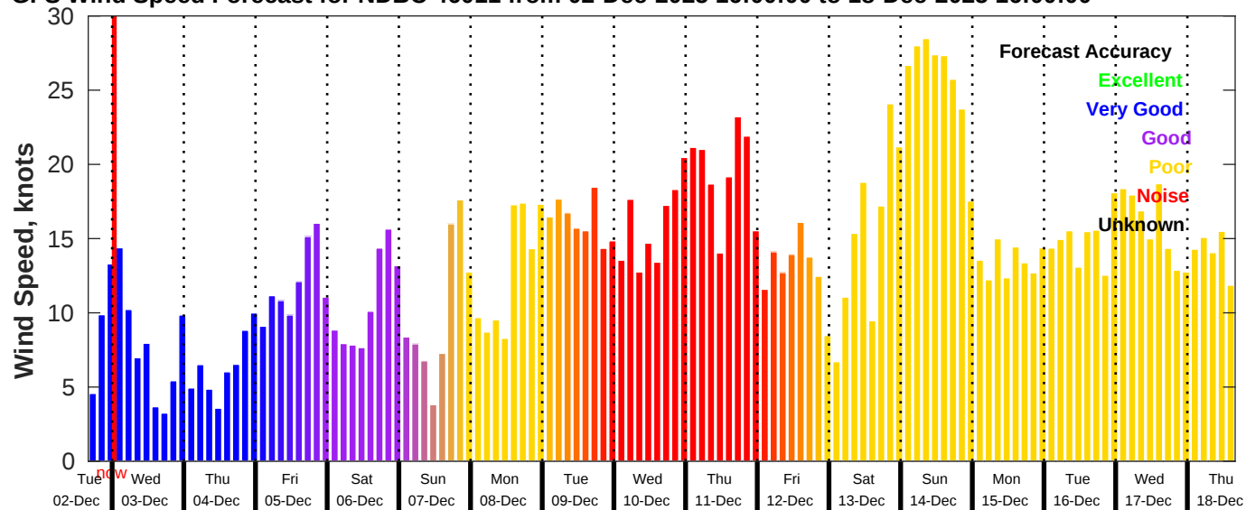
GFS Wind Speed Forecast for NDBC 46011 from 02-Dec-2025 16:00:00 to 18-Dec-2025 16:00:00
