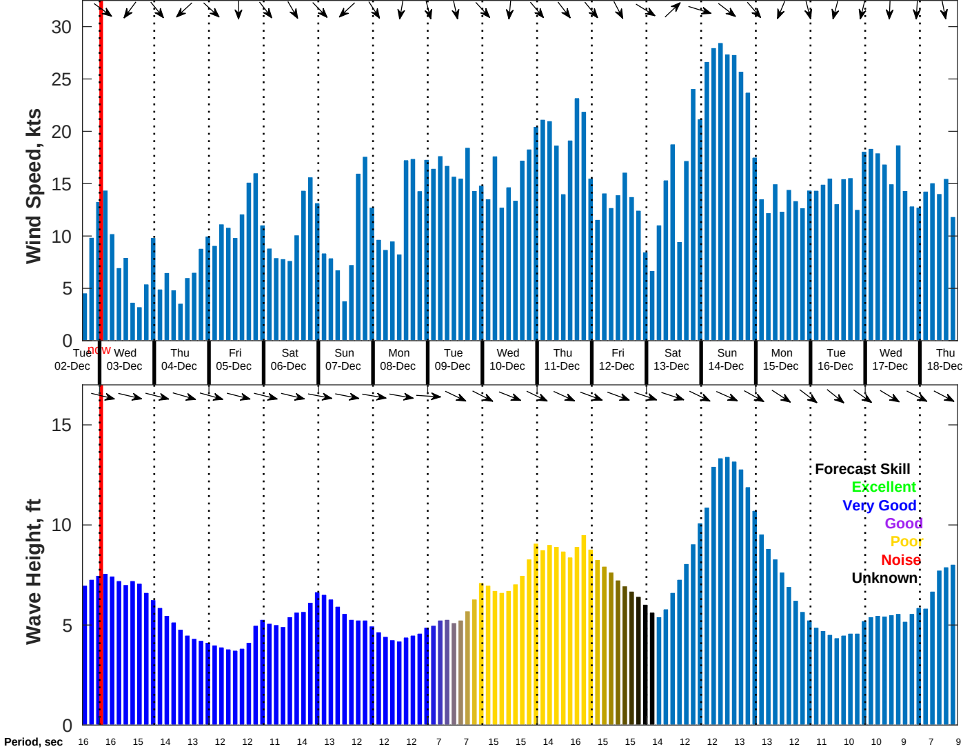
Wind & Wave Forecast for NDBC 46011 from 02-Dec-2025 16:00:00 to 18-Dec-2025 16:00:00
