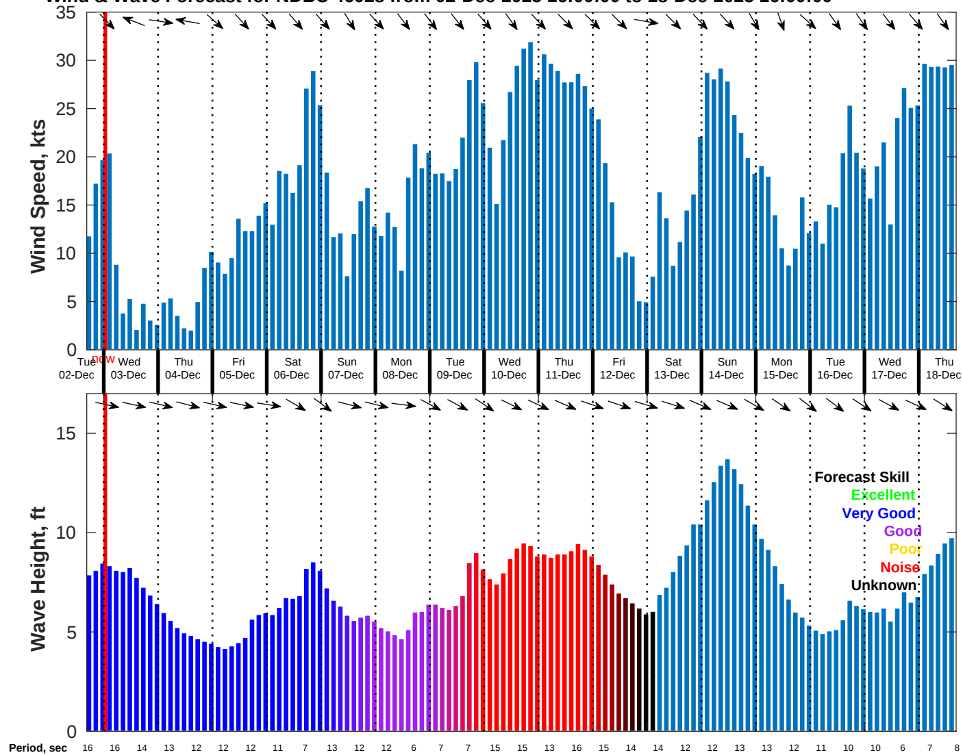
Wind & Wave Forecast for NDBC 46028 from 02-Dec-2025 16:00:00 to 18-Dec-2025 16:00:00
