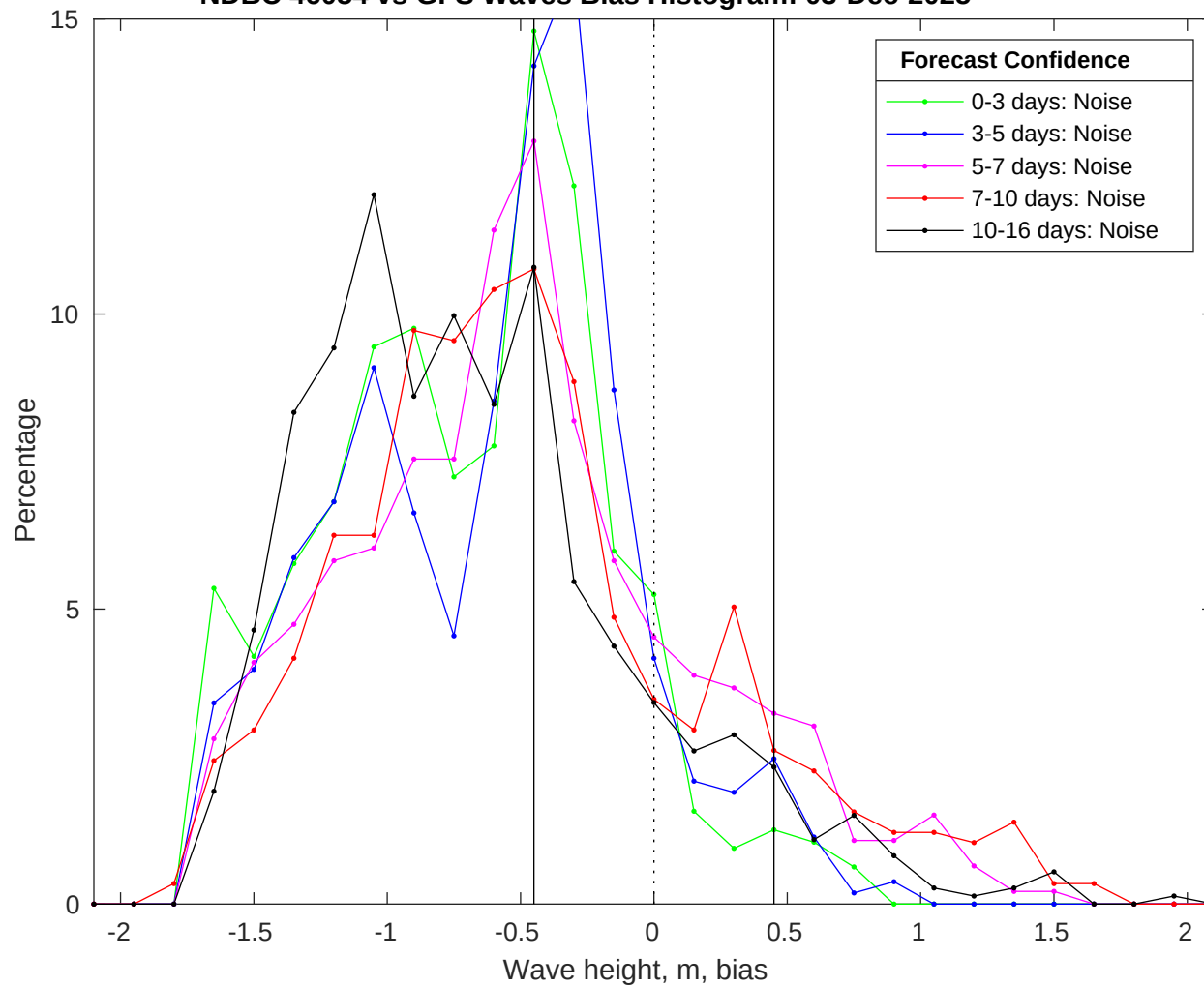
NDBC 46054 vs GFS Waves Bias Histogram: 03-Dec-2025
