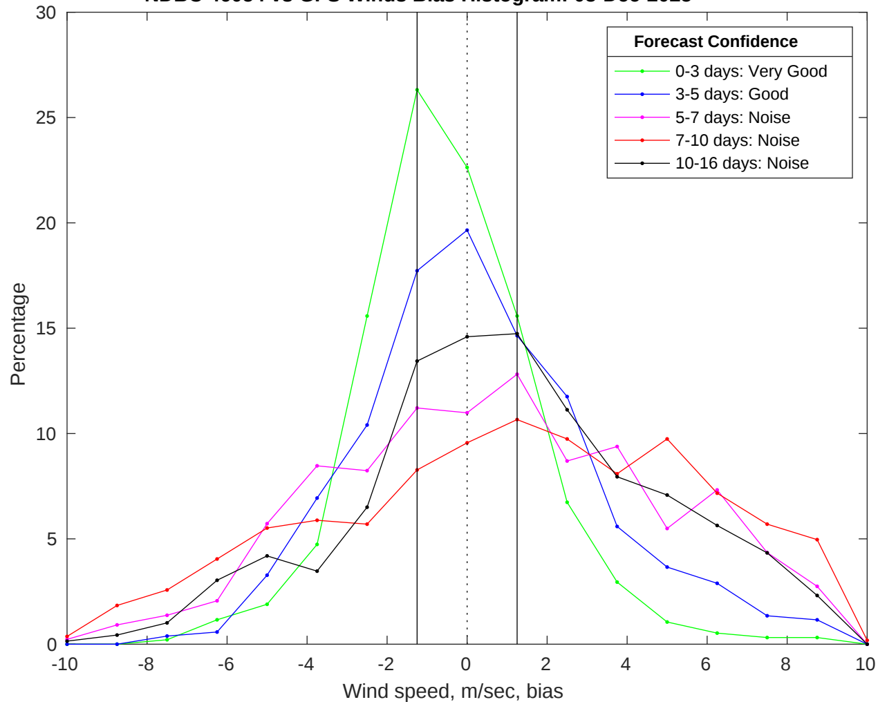
NDBC 46054 vs GFS Winds Bias Histogram: 03-Dec-2025
