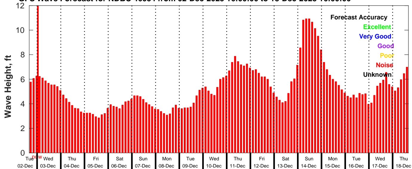
GFS Wave Forecast for NDBC 46054 from 02-Dec-2025 16:00:00 to 18-Dec-2025 16:00:00
