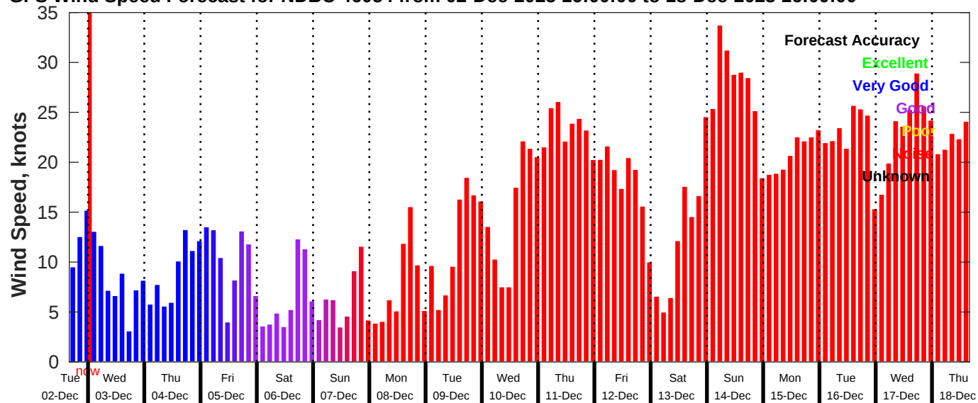
GFS Wind Speed Forecast for NDBC 46054 from 02-Dec-2025 16:00:00 to 18-Dec-2025 16:00:00
