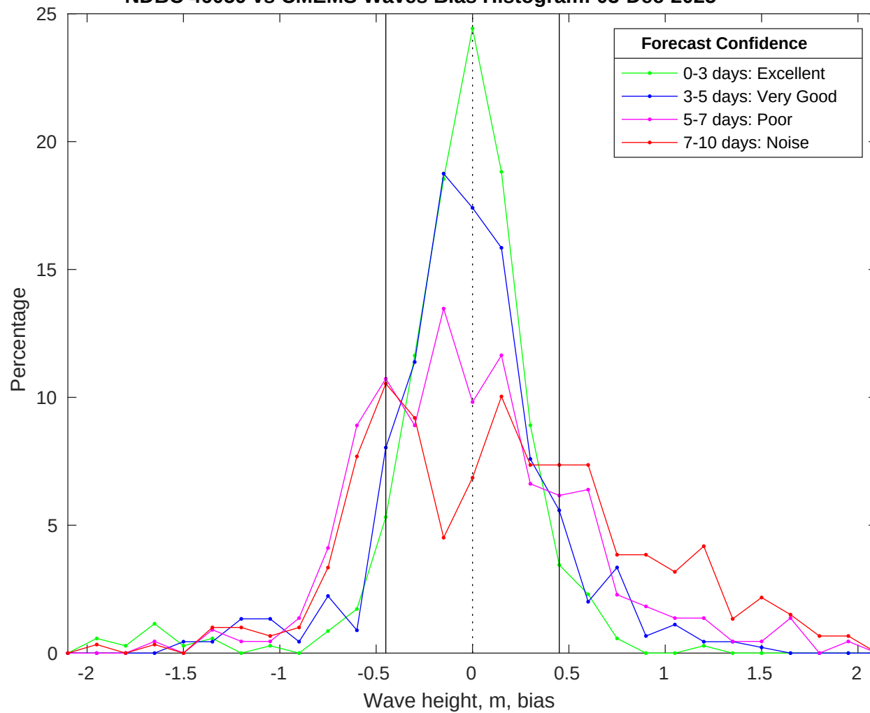
NDBC 46059 vs CMEMS Waves Bias Histogram: 03-Dec-2025
