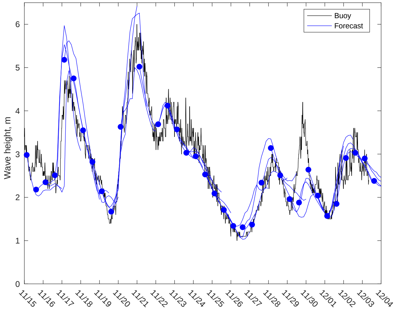
NDBC 46059 vs GFS Waves: 3 to 5 day forecast
