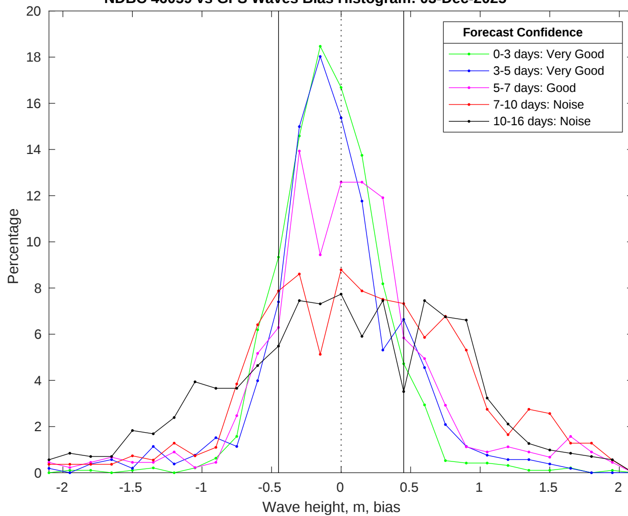
NDBC 46059 vs GFS Waves Bias Histogram: 03-Dec-2025
