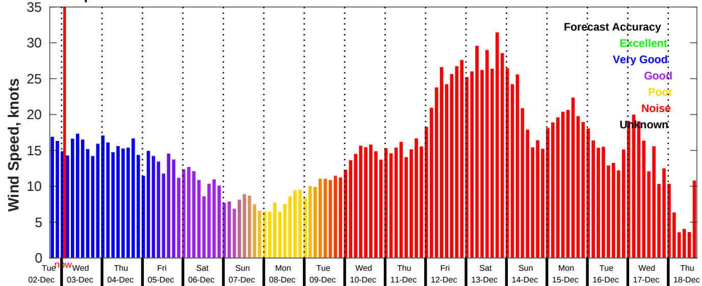
GFS Wind Speed Forecast for NDBC 46059 from 02-Dec-2025 17:00:00 to 18-Dec-2025 17:00:00
