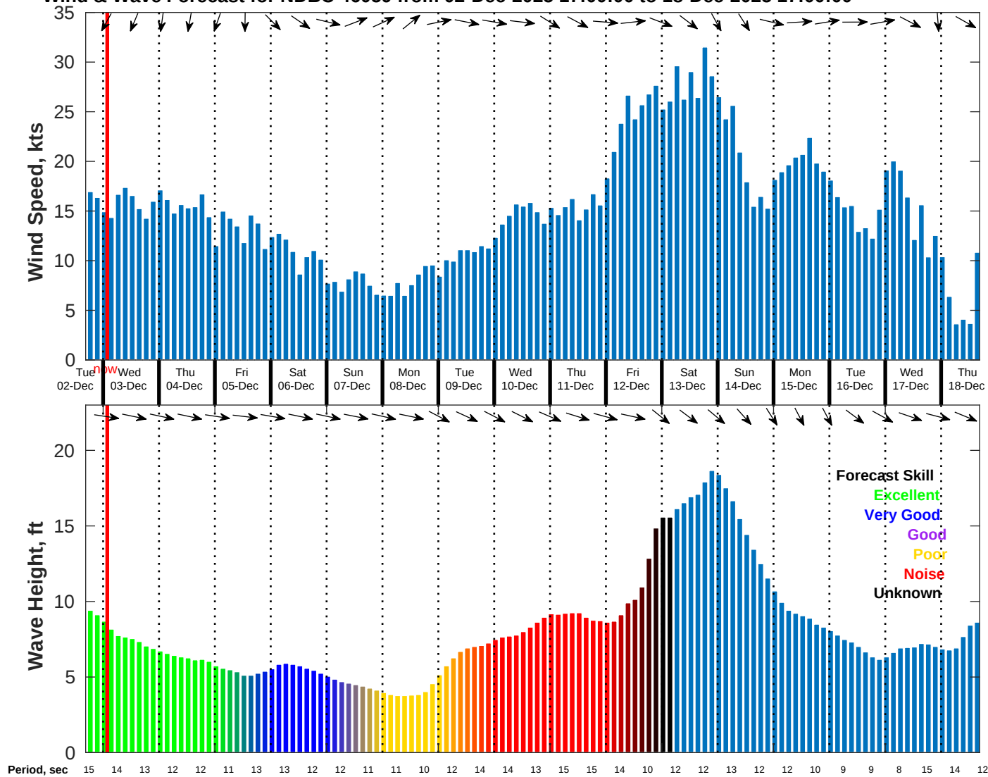
Wind & Wave Forecast for NDBC 46059 from 02-Dec-2025 17:00:00 to 18-Dec-2025 17:00:00
