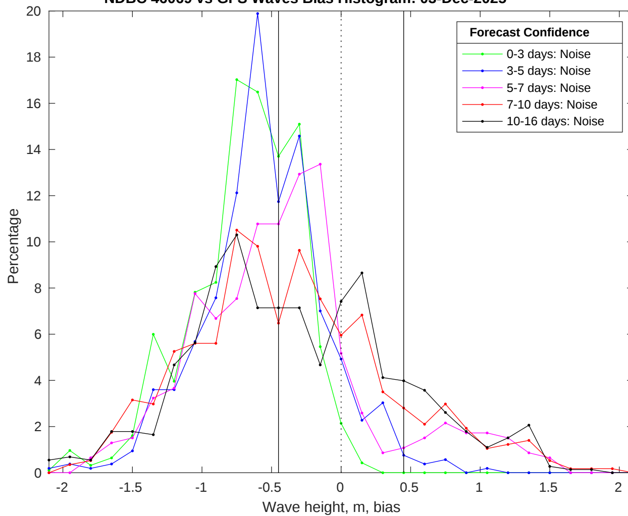
NDBC 46069 vs GFS Waves Bias Histogram: 03-Dec-2025
