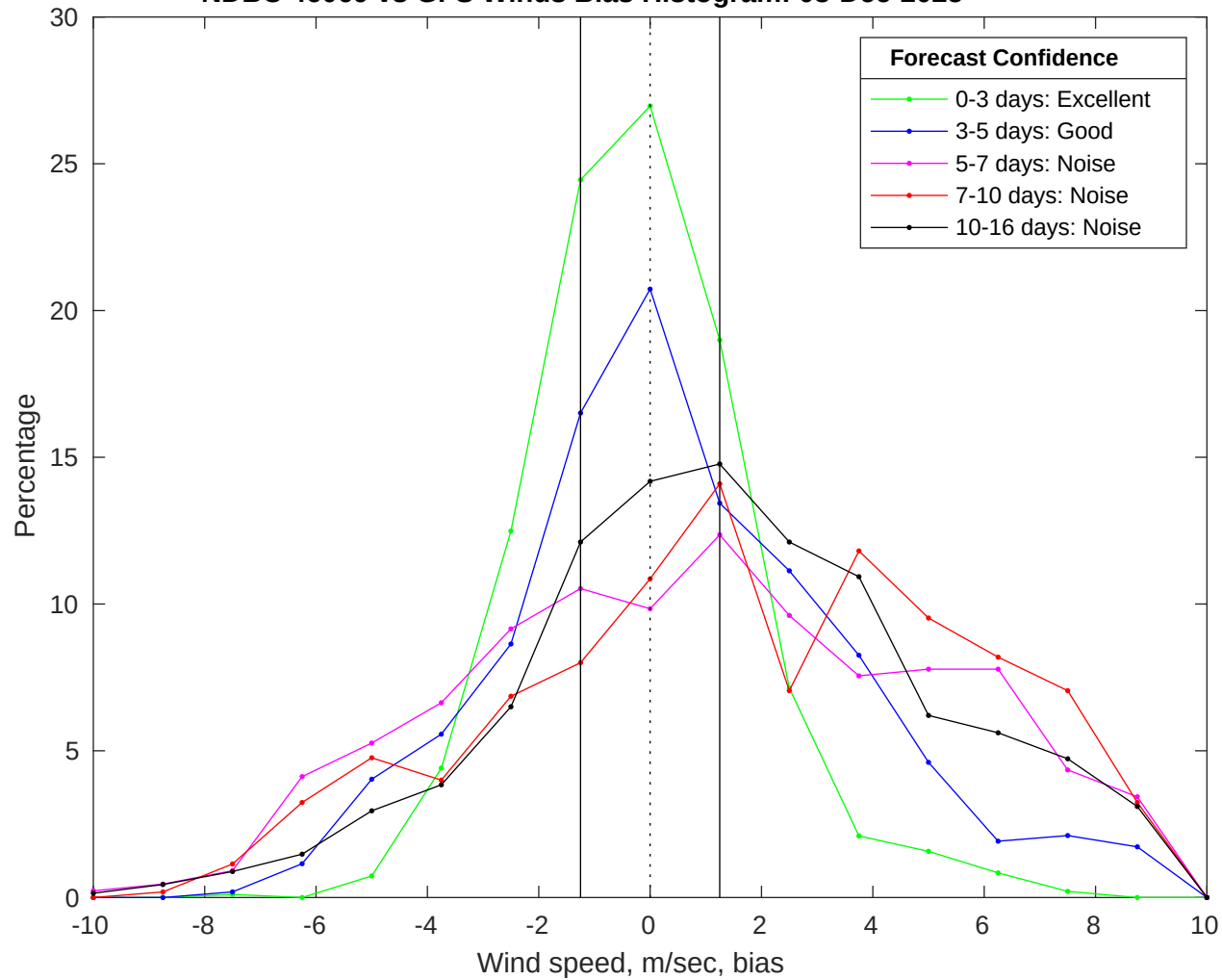
NDBC 46069 vs GFS Winds Bias Histogram: 03-Dec-2025
