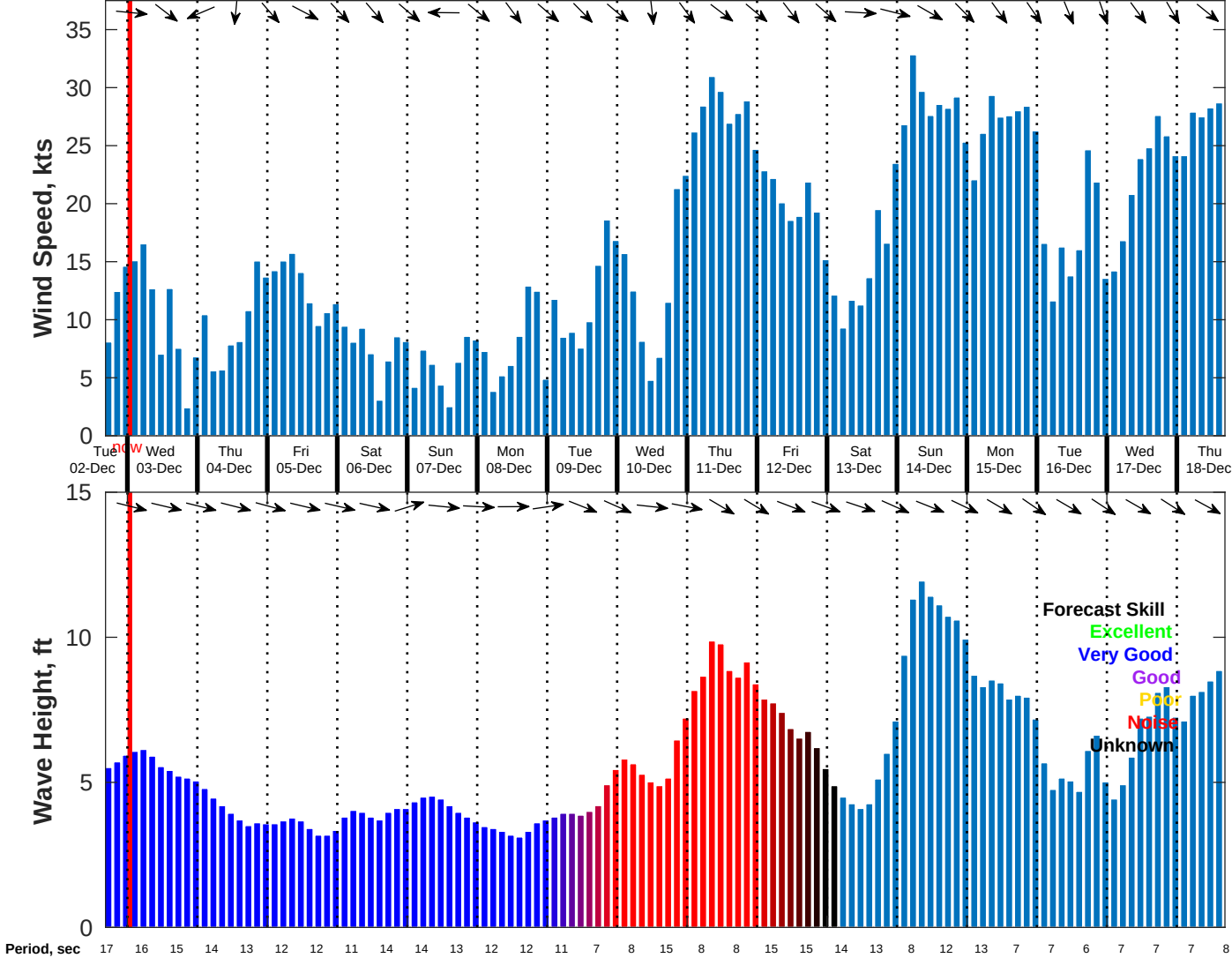
Wind & Wave Forecast for NDBC 46069 from 02-Dec-2025 16:00:00 to 18-Dec-2025 16:00:00
