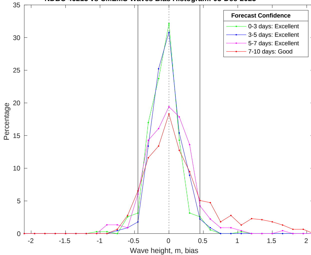
NDBC 46215 vs CMEMS Waves Bias Histogram: 03-Dec-2025
