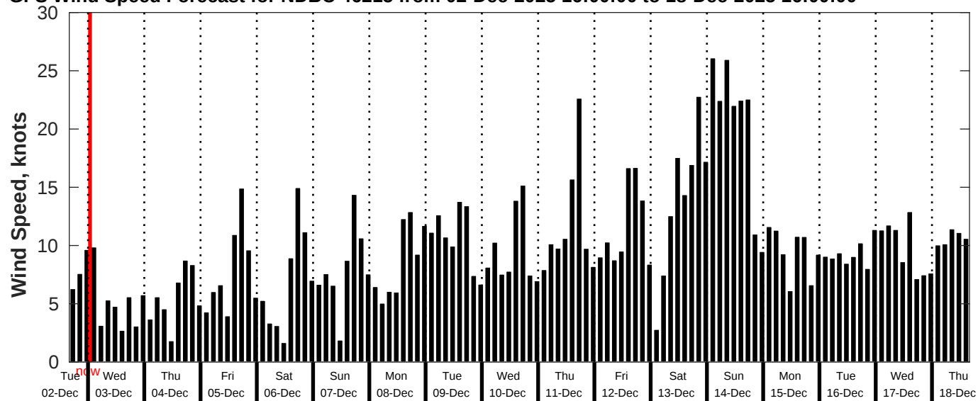
GFS Wind Speed Forecast for NDBC 46215 from 02-Dec-2025 16:00:00 to 18-Dec-2025 16:00:00
