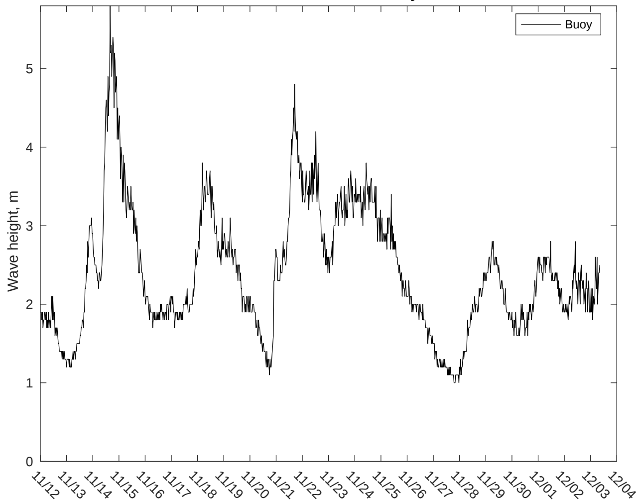
NDBC 46259 vs CMEMS Waves: 10 to 16 day forecast
