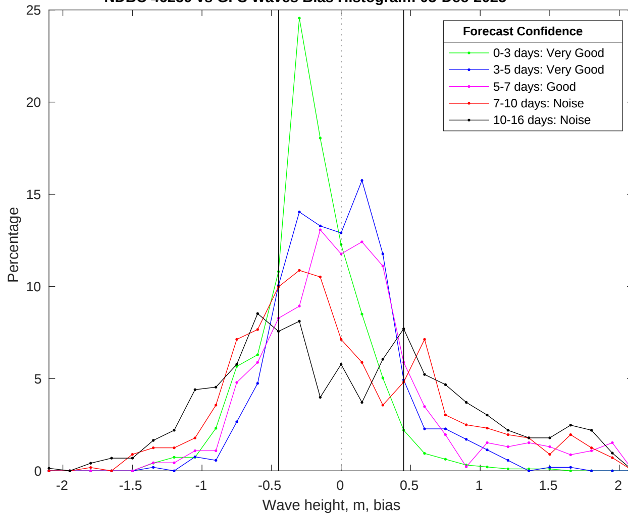
NDBC 46259 vs GFS Waves Bias Histogram: 03-Dec-2025
