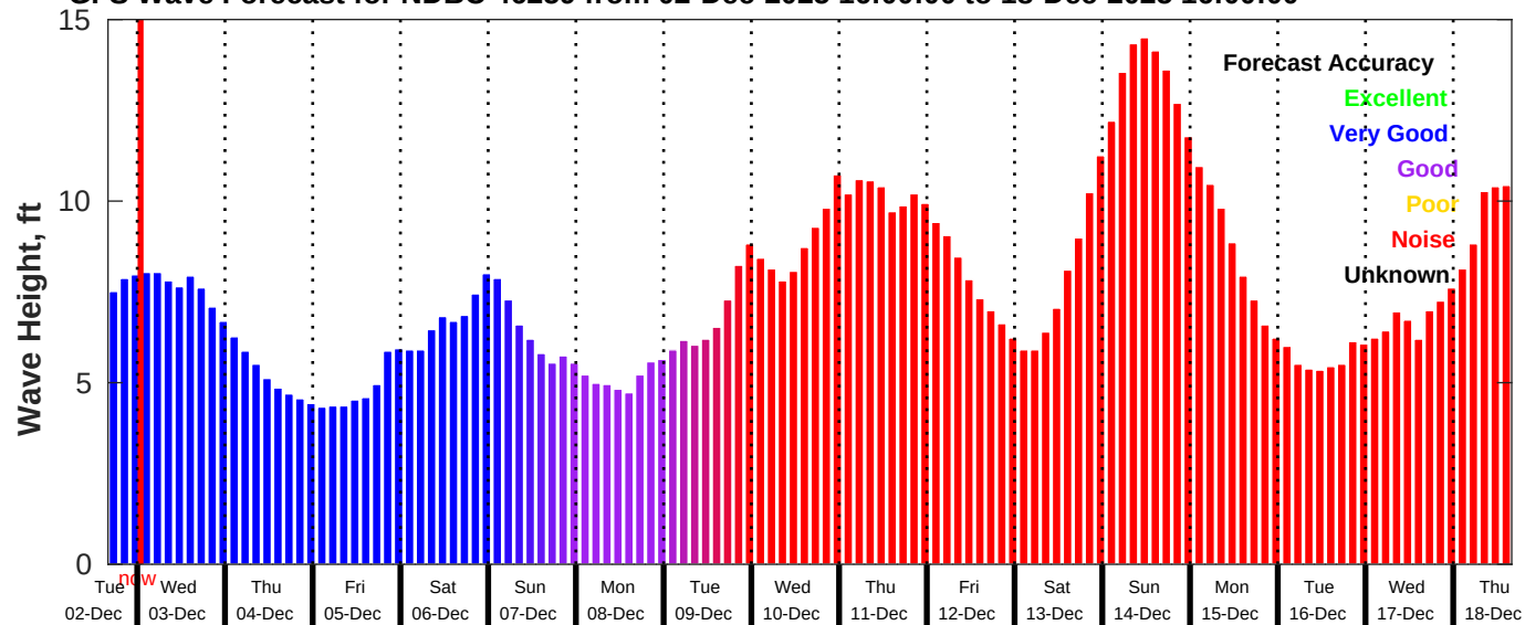
GFS Wave Forecast for NDBC 46259 from 02-Dec-2025 16:00:00 to 18-Dec-2025 16:00:00
