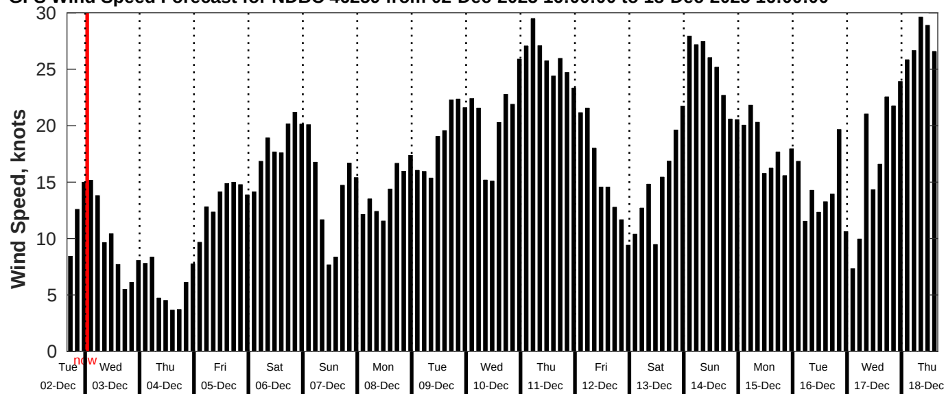
GFS Wind Speed Forecast for NDBC 46259 from 02-Dec-2025 16:00:00 to 18-Dec-2025 16:00:00
