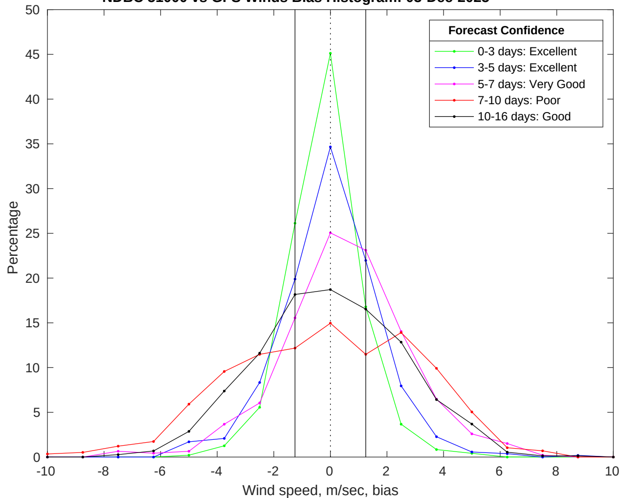
NDBC 51000 vs GFS Winds Bias Histogram: 03-Dec-2025
