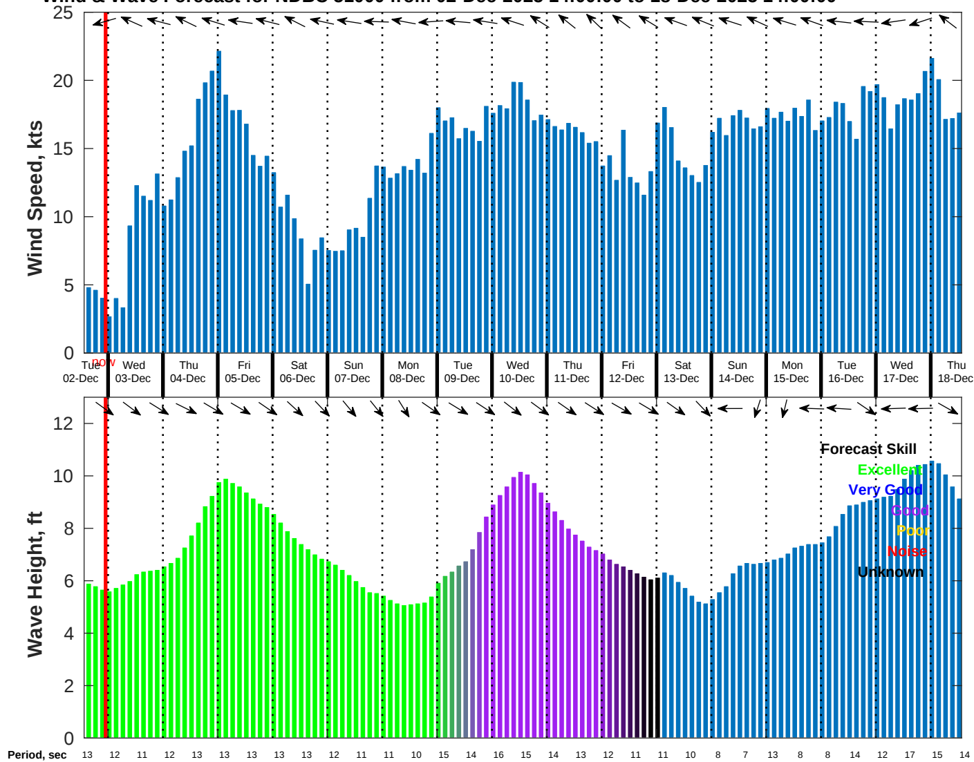
Wind & Wave Forecast for NDBC 51000 from 02-Dec-2025 14:00:00 to 18-Dec-2025 14:00:00
