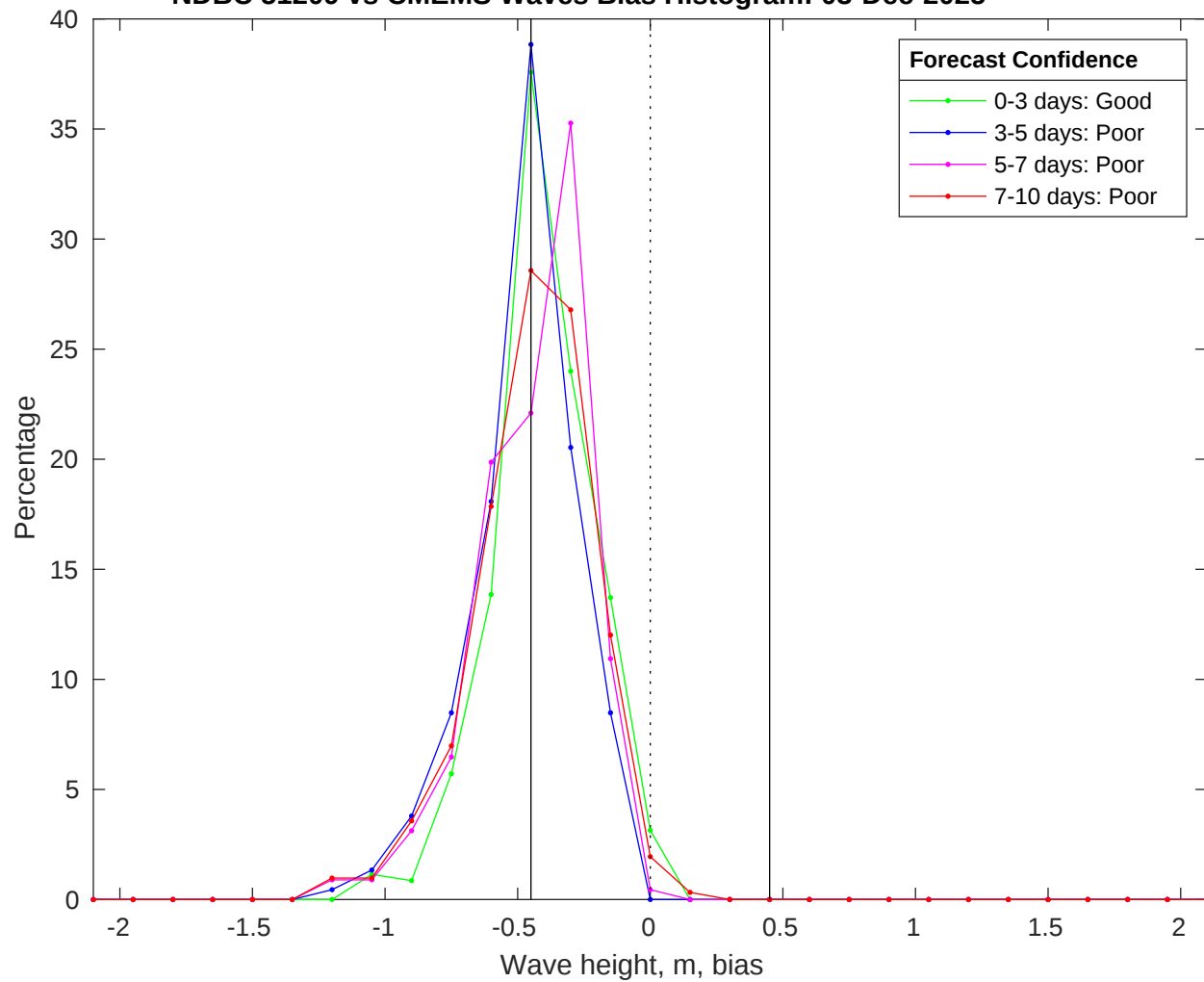
NDBC 51209 vs CMEMS Waves Bias Histogram: 03-Dec-2025
