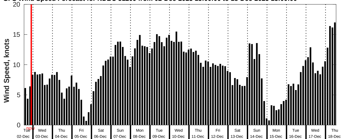
GFS Wind Speed Forecast for NDBC 51209 from 02-Dec-2025 13:00:00 to 18-Dec-2025 13:00:00
