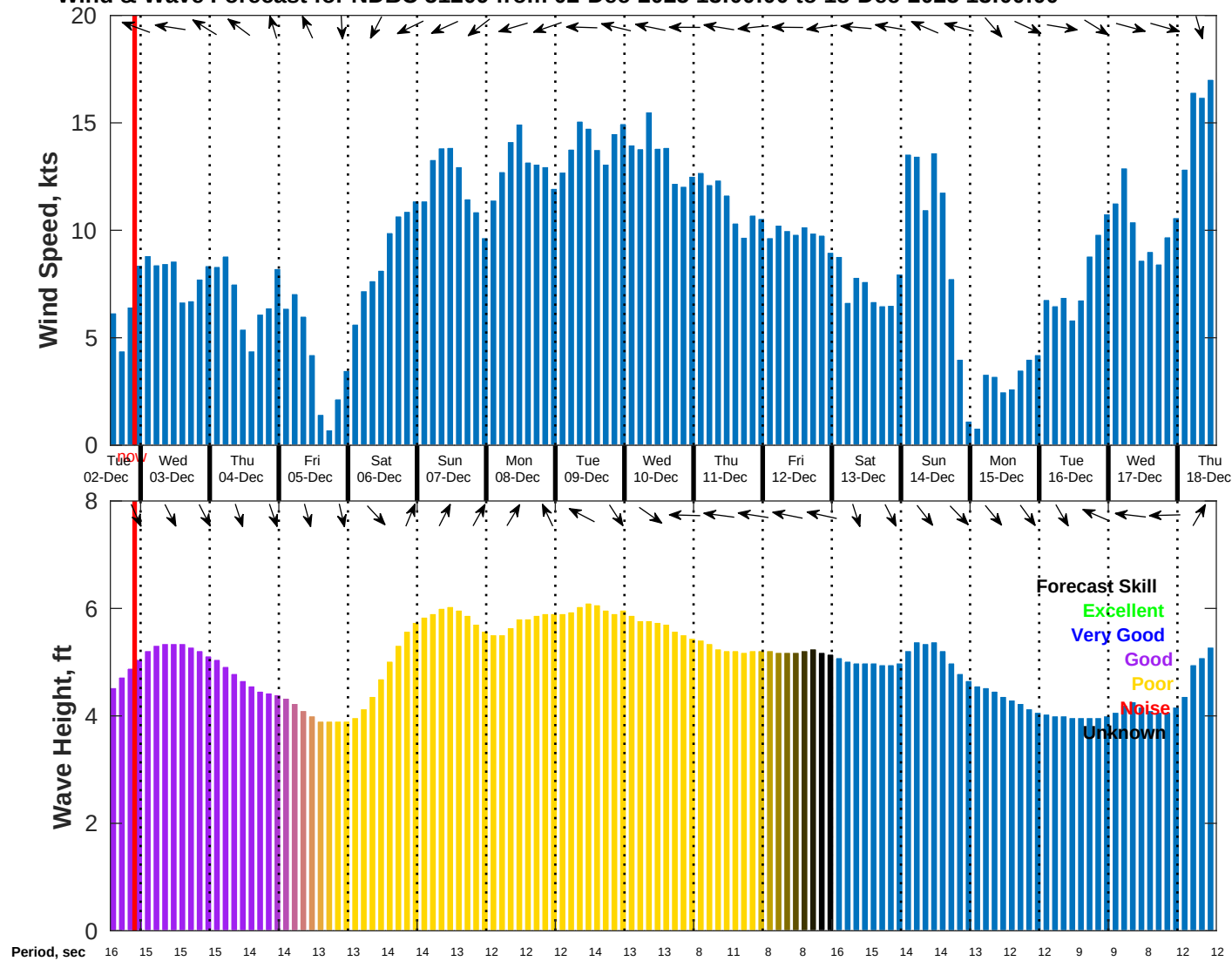
Wind & Wave Forecast for NDBC 51209 from 02-Dec-2025 13:00:00 to 18-Dec-2025 13:00:00
