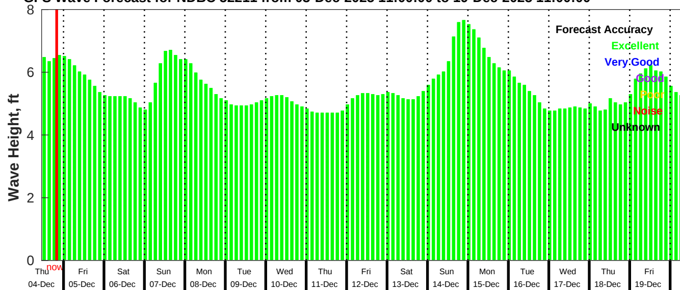
GFS Wave Forecast for NDBC 52211 from 03-Dec-2025 11:00:00 to 19-Dec-2025 11:00:00
