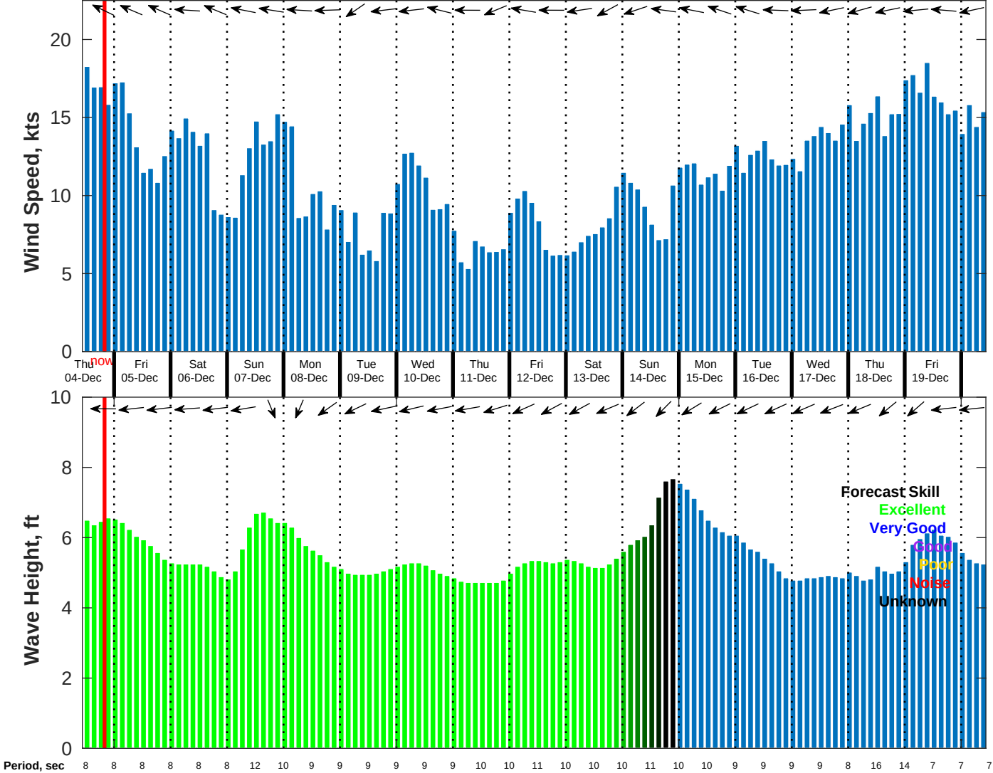
Wind & Wave Forecast for NDBC 52211 from 03-Dec-2025 11:00:00 to 19-Dec-2025 11:00:00
