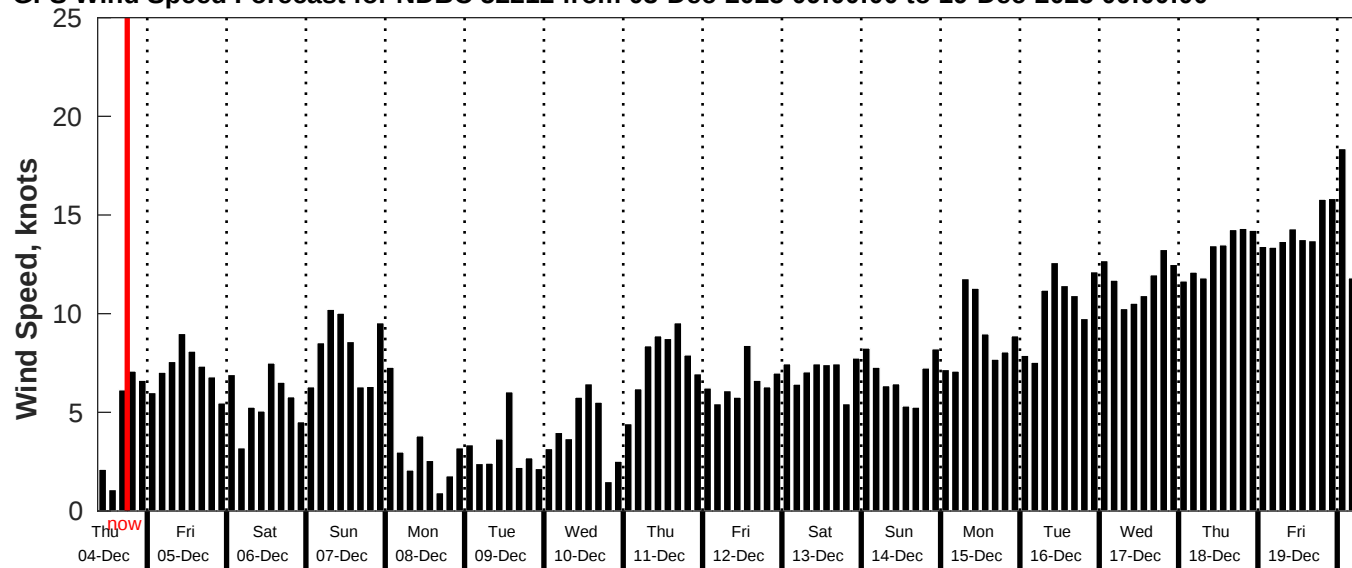
GFS Wind Speed Forecast for NDBC 52212 from 03-Dec-2025 09:00:00 to 19-Dec-2025 09:00:00
