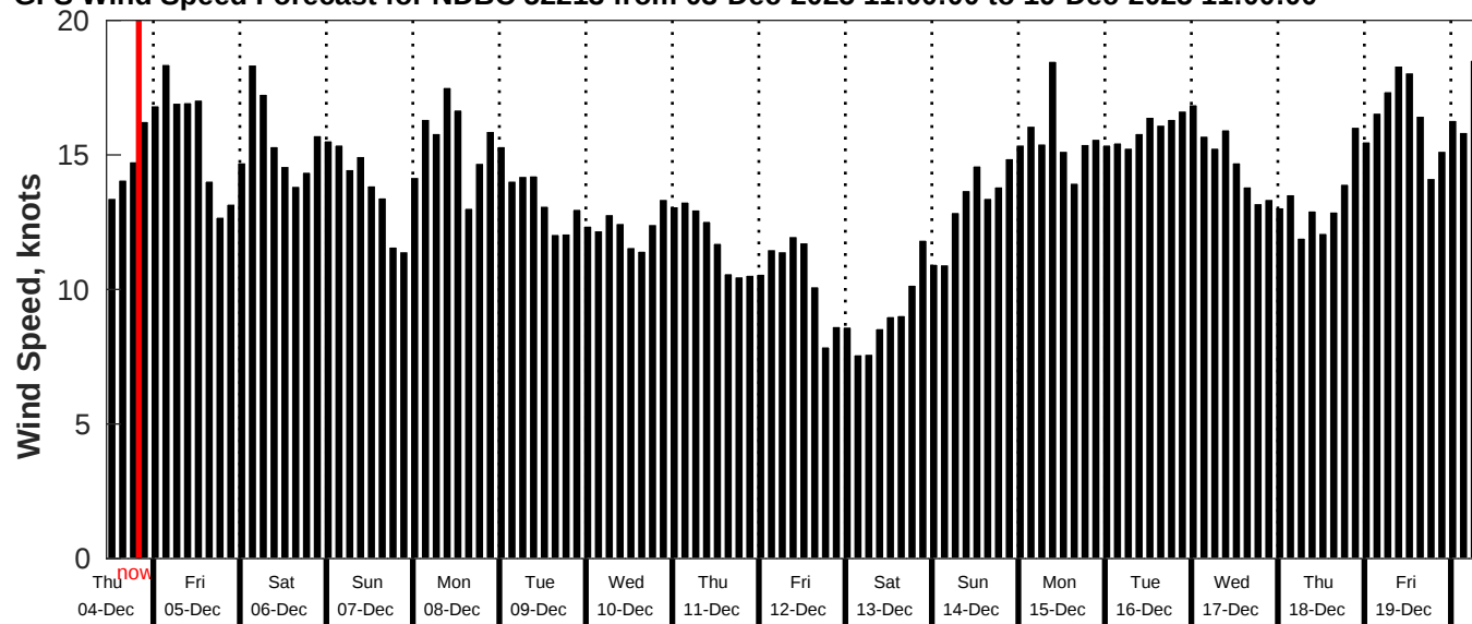
GFS Wind Speed Forecast for NDBC 52213 from 03-Dec-2025 11:00:00 to 19-Dec-2025 11:00:00
