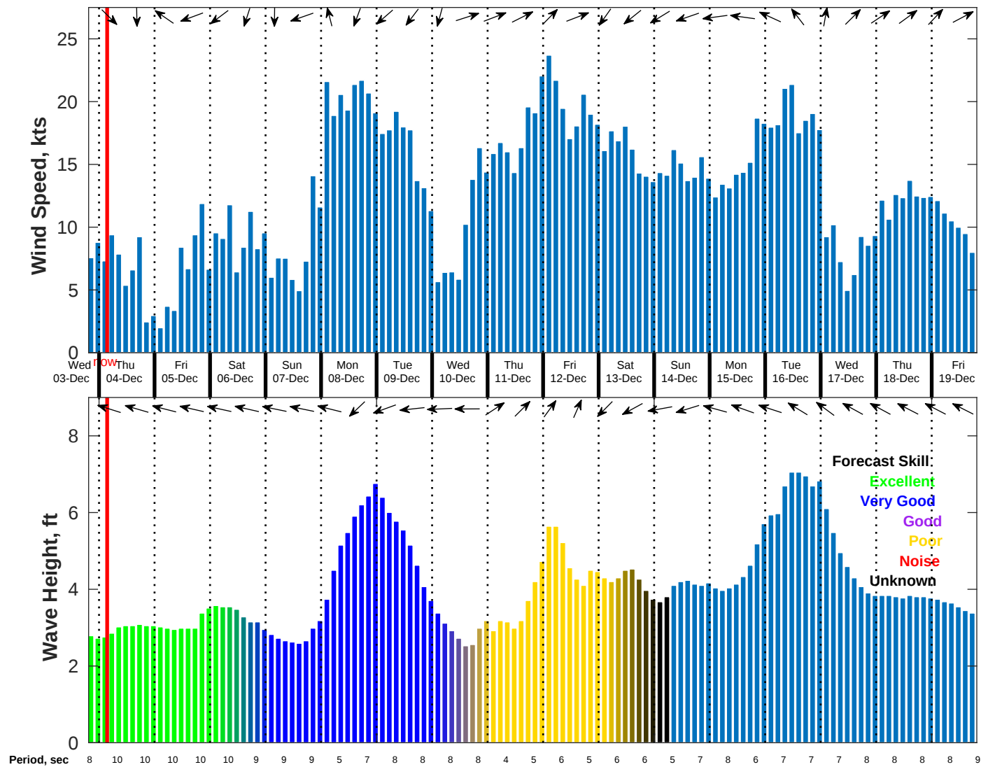
Wind & Wave Forecast for NDBC 41004 from 03-Dec-2025 19:00:00 to 19-Dec-2025 19:00:00
