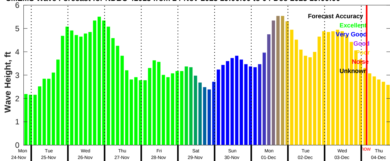
CMEMS Wave Forecast for NDBC 41013 from 24-Nov-2025 19:00:00 to 04-Dec-2025 19:00:00
