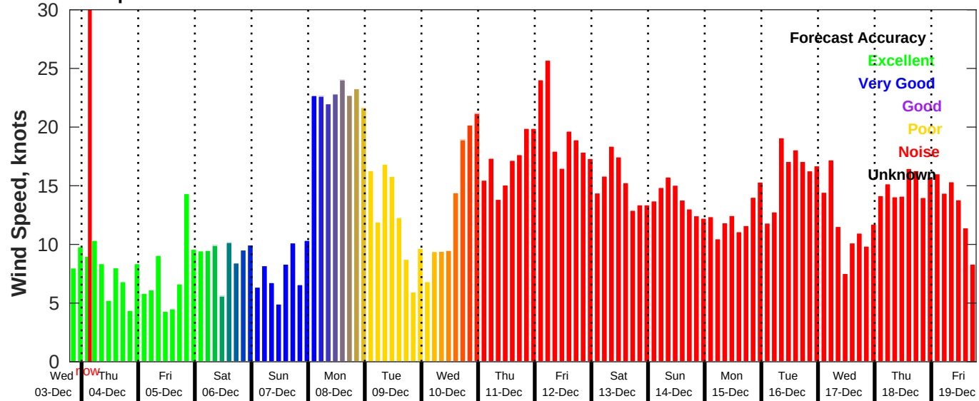
GFS Wind Speed Forecast for NDBC 41013 from 03-Dec-2025 19:00:00 to 19-Dec-2025 19:00:00
