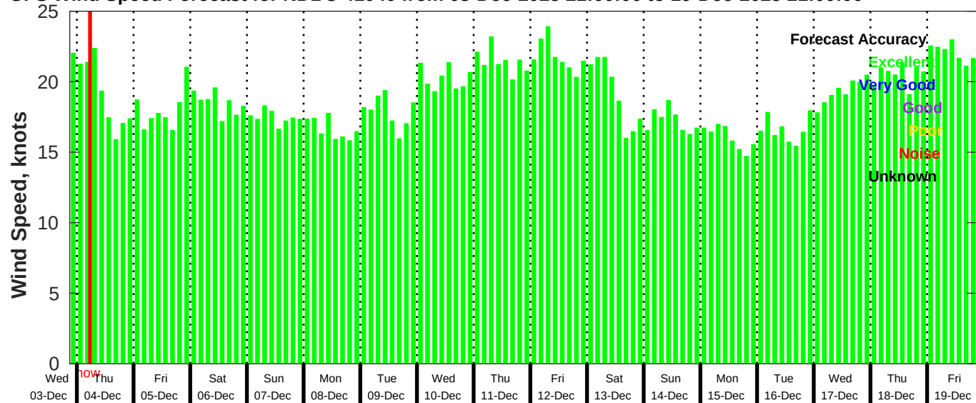
GFS Wind Speed Forecast for NDBC 41040 from 03-Dec-2025 21:00:00 to 19-Dec-2025 21:00:00
