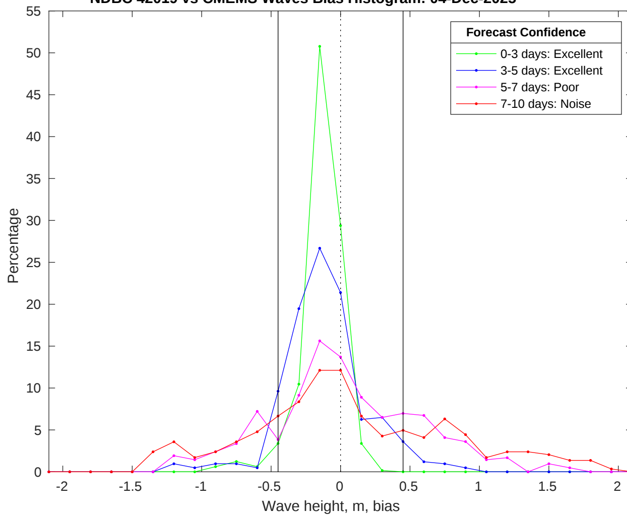
NDBC 42019 vs CMEMS Waves Bias Histogram: 04-Dec-2025
