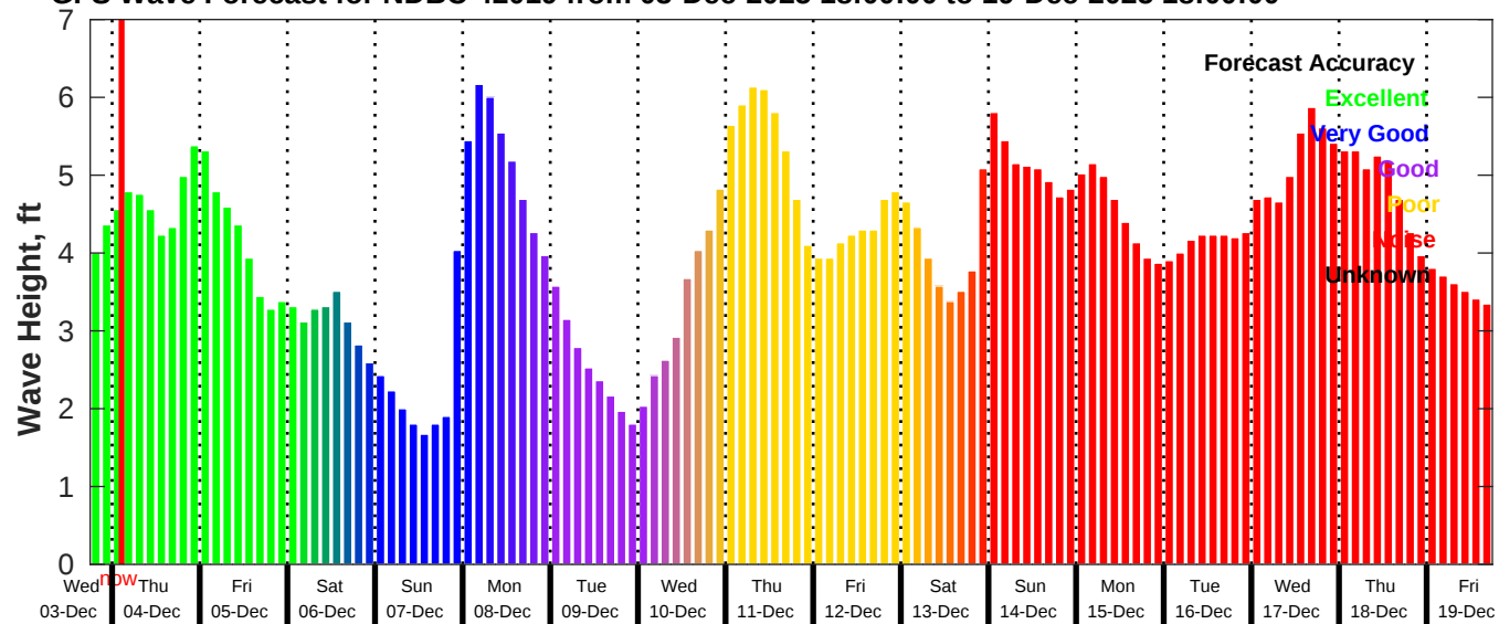
GFS Wave Forecast for NDBC 42019 from 03-Dec-2025 18:00:00 to 19-Dec-2025 18:00:00
