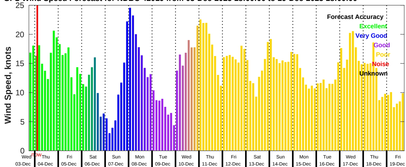
GFS Wind Speed Forecast for NDBC 42019 from 03-Dec-2025 18:00:00 to 19-Dec-2025 18:00:00
