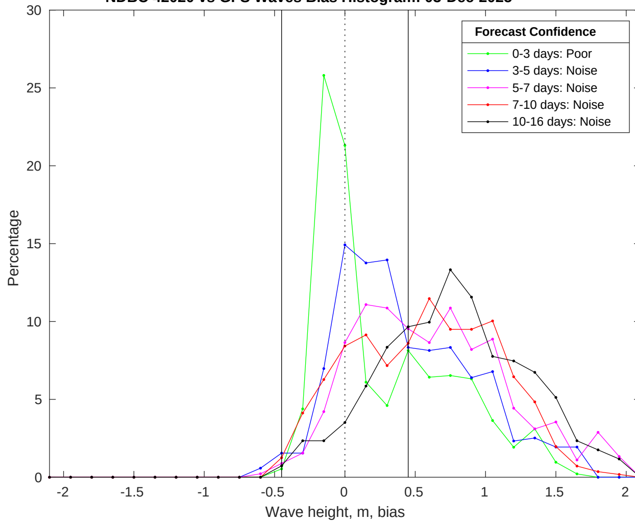
NDBC 42020 vs GFS Waves Bias Histogram: 03-Dec-2025
