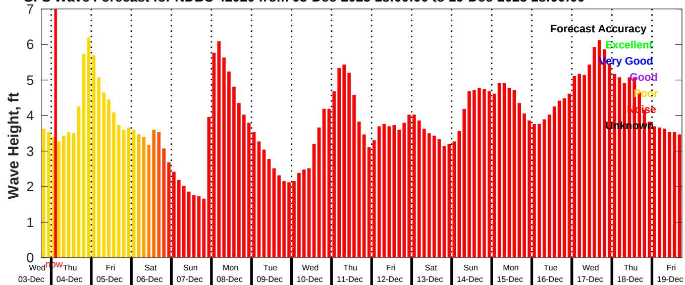
GFS Wave Forecast for NDBC 42020 from 03-Dec-2025 18:00:00 to 19-Dec-2025 18:00:00
