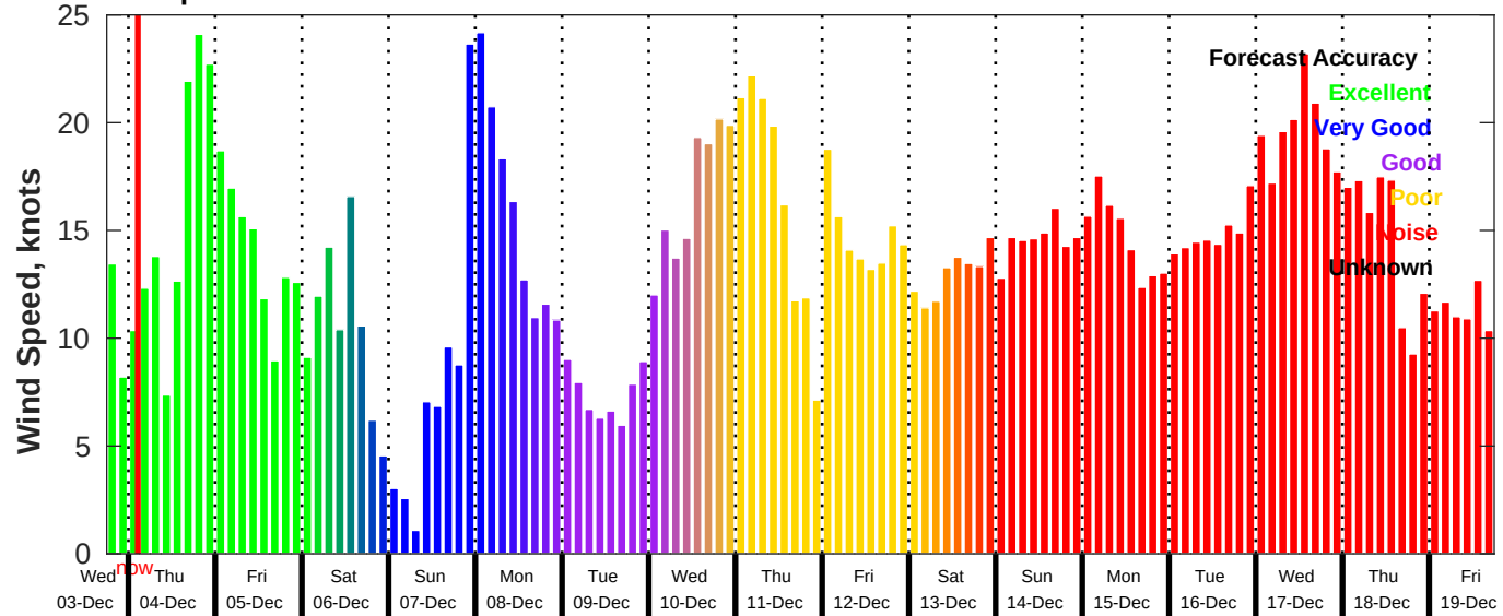
GFS Wind Speed Forecast for NDBC 42020 from 03-Dec-2025 18:00:00 to 19-Dec-2025 18:00:00
