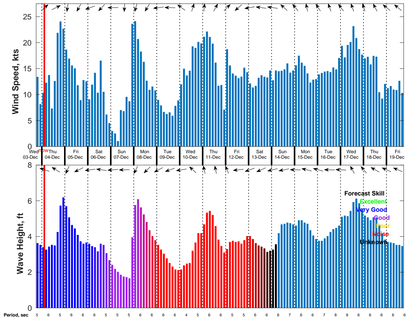
Wind & Wave Forecast for NDBC 42020 from 03-Dec-2025 18:00:00 to 19-Dec-2025 18:00:00
