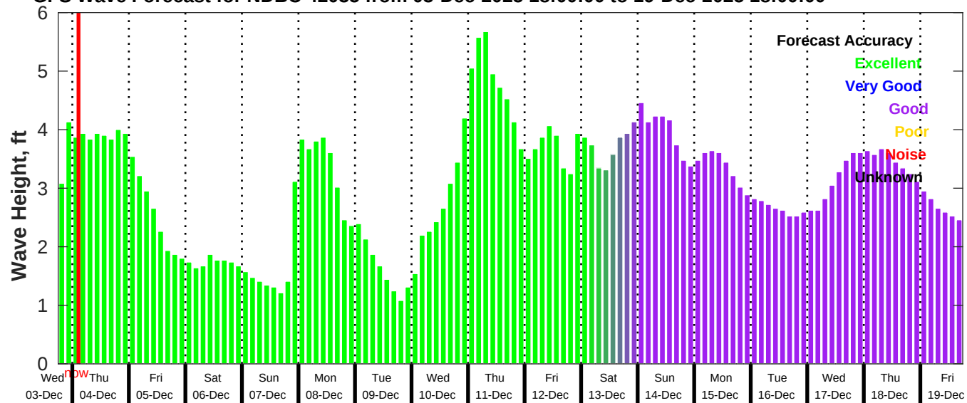
GFS Wave Forecast for NDBC 42035 from 03-Dec-2025 18:00:00 to 19-Dec-2025 18:00:00
